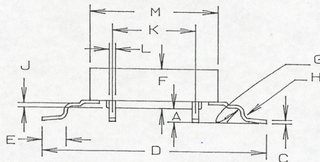
LID DOWN FORM SPECIFICATIONS
