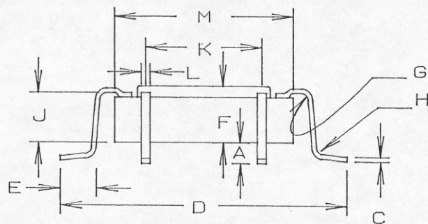
LID UP FORM SPECIFICATIONS
